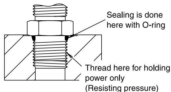
Fig. 6 – UNF port assembly
