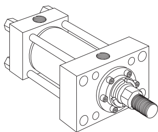
Style JJ Rectangular Head (NPPA Style ME5)
