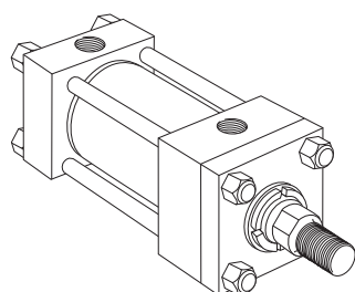
Style F Side Tapped Mounting (NFFPA Style MS4)
