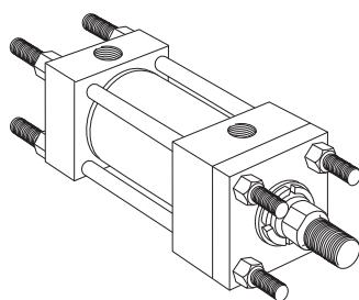
Style TD Tie Rods Extended Both Ends (NFA Style MX1)
