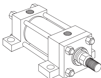
Style C Side Lug Mounting (NFFPA Style MS2)
