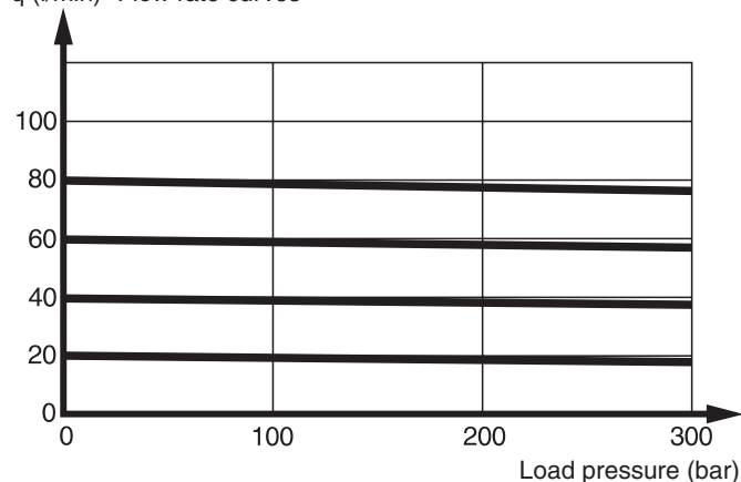
q (l/min) Flow rate curves
