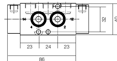
Dimensions Reference 9
