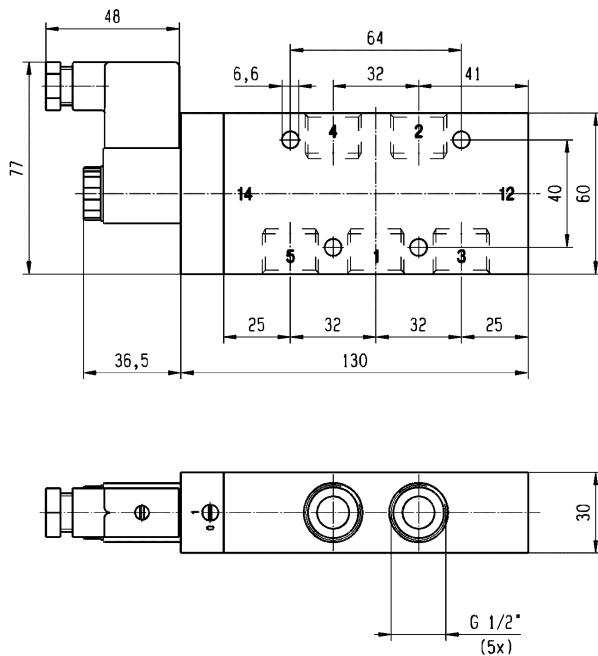
Dimensions Reference 22
