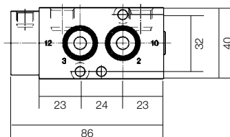
Dimensions Reference 7
