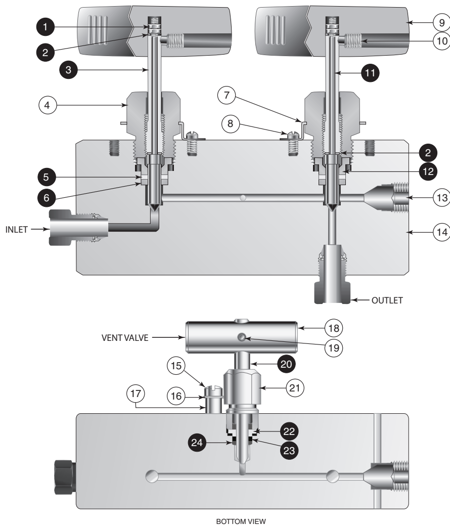
BOTTOM VIEW
