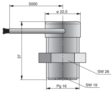
Dimensions (mm) – Sensing Head
