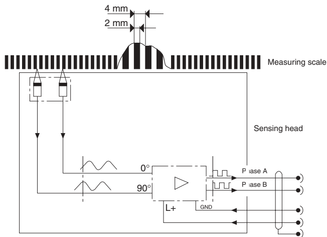
Connection diagram – Sensing head
