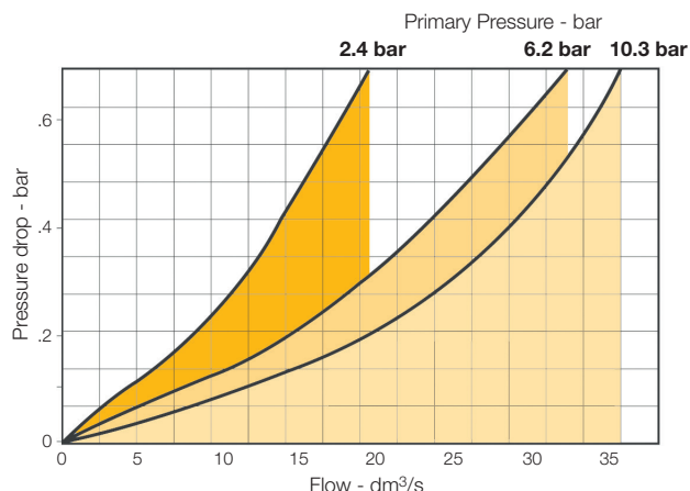
Flow Characteristics - 1/2 Inch Ports PF11-04DJSS
