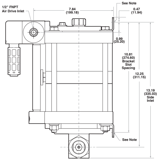
Right View
