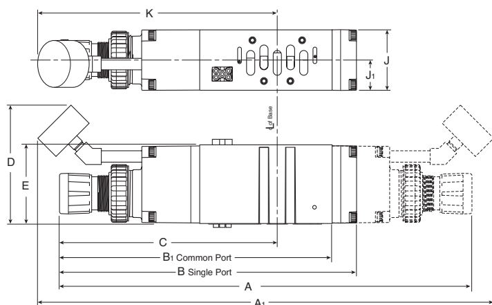
H2 &amp; H3 Series Sandwich Regulator, Dimensions
