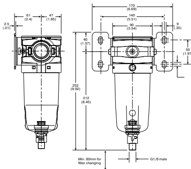
(3/4") Filter
