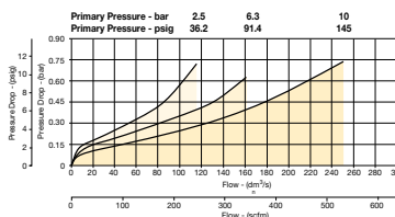
(3/4") Lubricator
