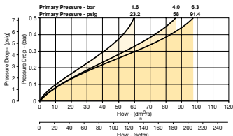
P33LA 3/4" Lubricator
