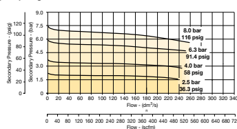
(3/4") Regulator
