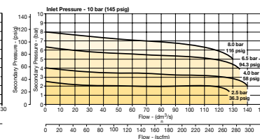
P33EA 3/4" Filter/Regulator
