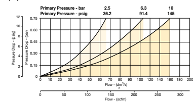
(1") Filter
