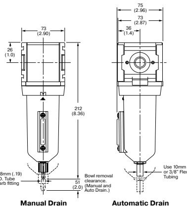
P33FA 1/2" Filter
