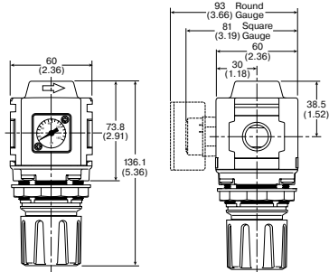
P32RB 1/2" Regulator
